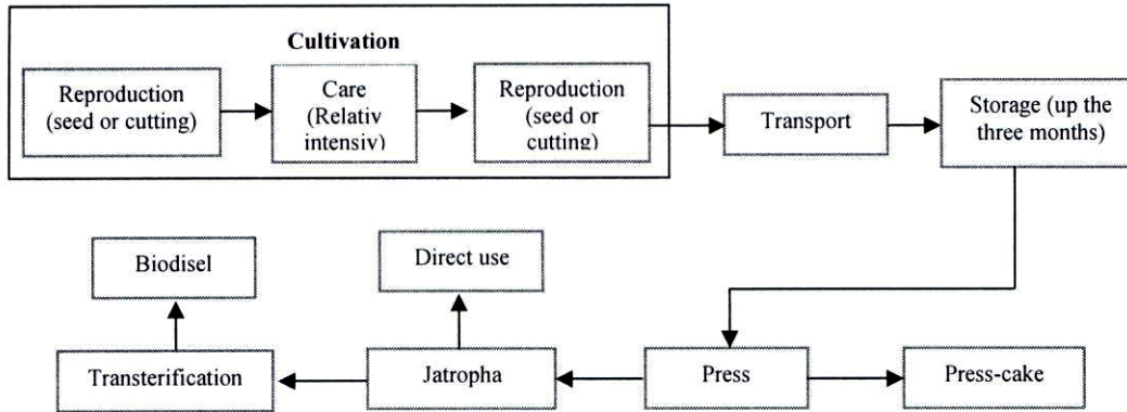
Figure 2: General process chain for the biodiesel production from Jatropha curcas
